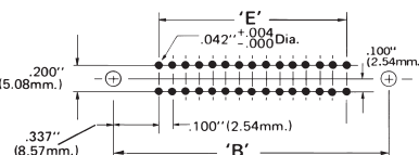
DUAL PC CONTACT PATTERN
