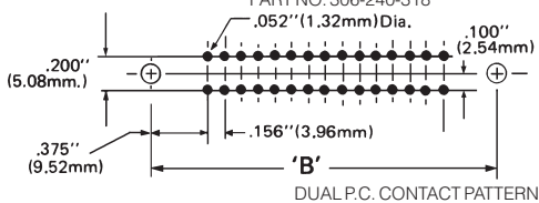
SINGLE-READOUT DUAL-READOUT POLARIZING INSERTS: BETWEEN CONTACT PART NO. 306-240-318 IN CONTACT PART NO. 307-240-328
