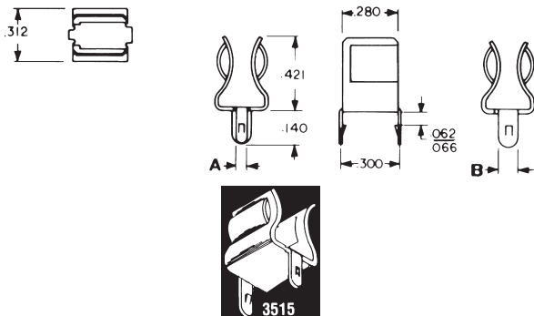
.020 BRASS, TIN PLATE. FOR 1/4" DIA. FUSES.
