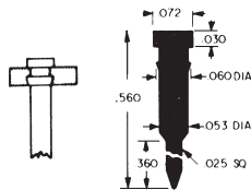
I.C. SOCKET CONTACTS
