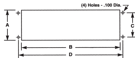
PANEL CUTOUT DIMENSIONS
