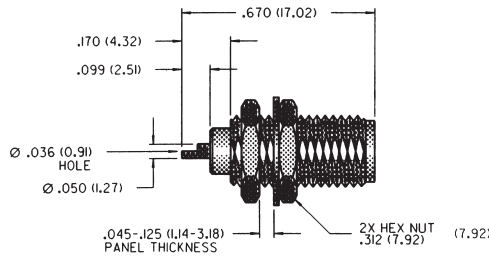
SMA 50 OHM FRONT MOUNT BULKHEAD JACK RECEPTACLE
