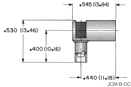
FLEXIBLE CABLE—RIGHT ANGLE CRIMP TYPE PLUG SMB 50 OHM—DIE CAST
