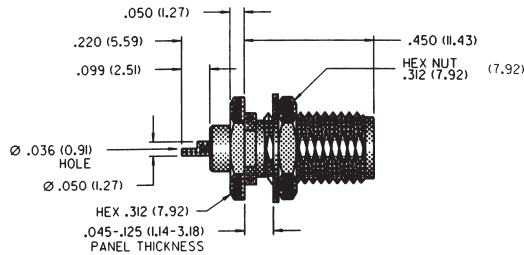
SMA 50 OHM REAR MOUNT BULKHEAD JACK RECEPTACLE
