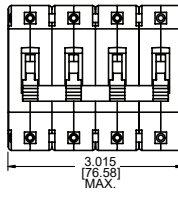
Panel Mounting Detail
