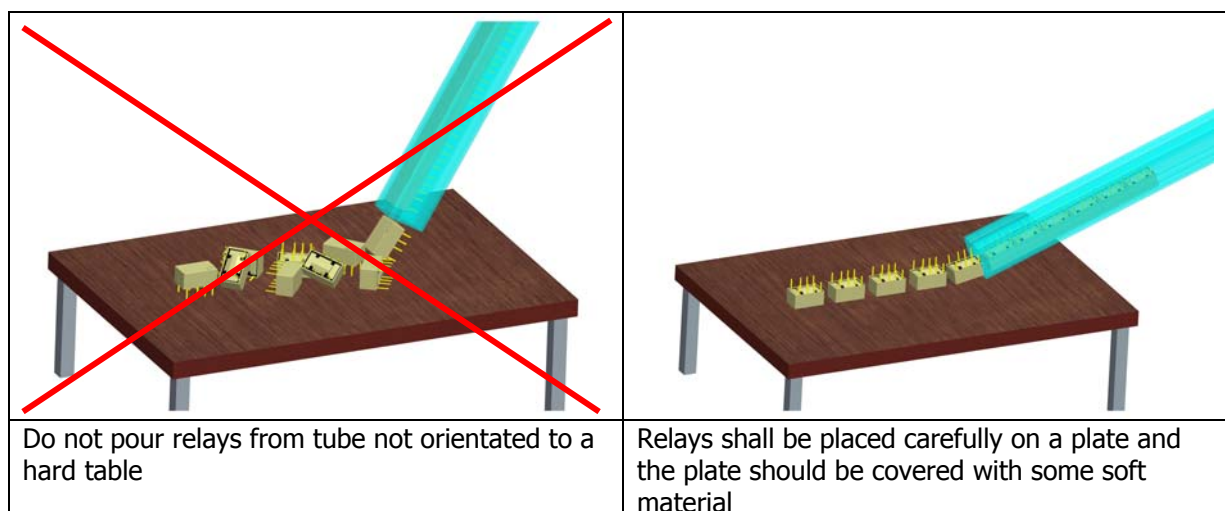
Fig. 6: Proper and improper release of relays from the tube.
