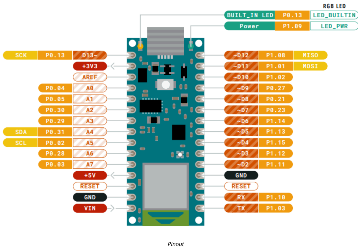
Pinout
