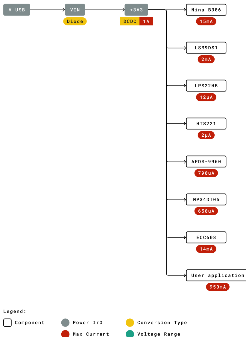
Power tree
