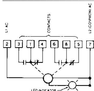
TYPICAL CIRCUIT
