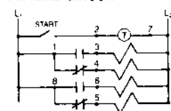
TYPICAL CIRCUIT
