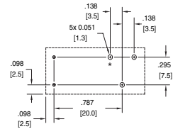
3.5mm SPACING 1 FORM C
