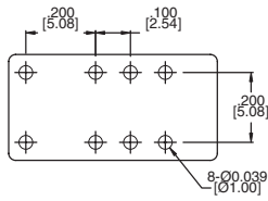
SINGLE SIDE STABLE & 1 COIL LATCHING
