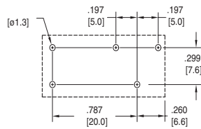
5.0mm SPACING FORM "C"
