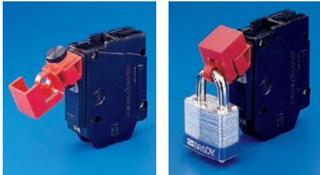
The Brady Clamp-On Circuit Breaker Lockout works on an extremely wide range of breakers.
