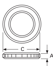
Knurled Facenut
