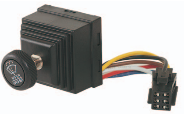
Rotary Wiper
