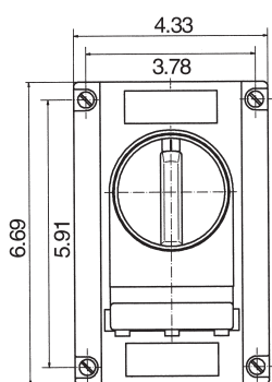
Figure 2 - 20 Amp, 3 Pole
