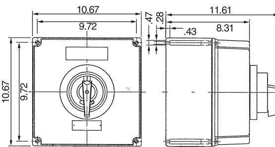
Figure 7 - 80 Amp, 6 Pole
