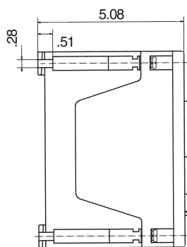
Figure 2 - 20 Amp, 3 Pole
