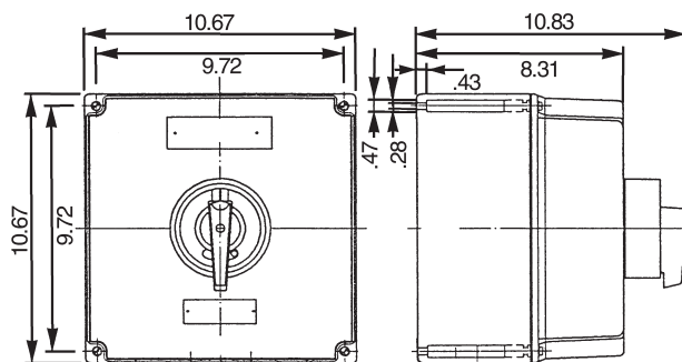
Figure 5 - 40 Amp, 6 Pole
