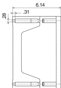
Figure 4 - 40 Amp, 3 Pole
