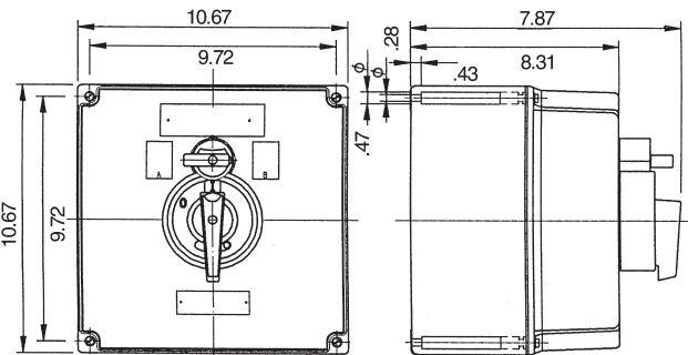
Figure 10 - 40 Amp, 6 Phase Variable Speed
