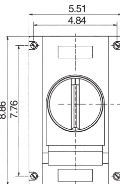
Figure 3 - 20 Amp, 6 Pole
