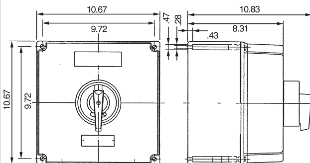
Figure 6 - 80 Amp, 3 Pole
