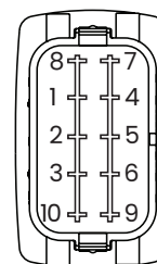
TERMINAL ARRANGMENT
