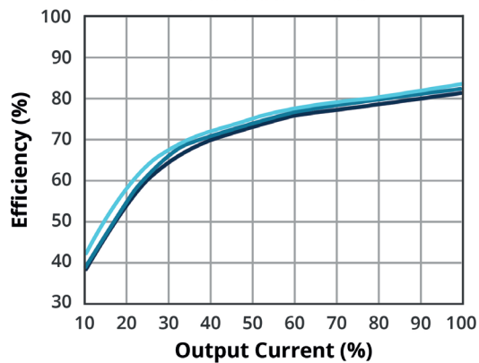
EFFICIENCY VS OUTPUT LOAD PCN1-S12-S15-S
