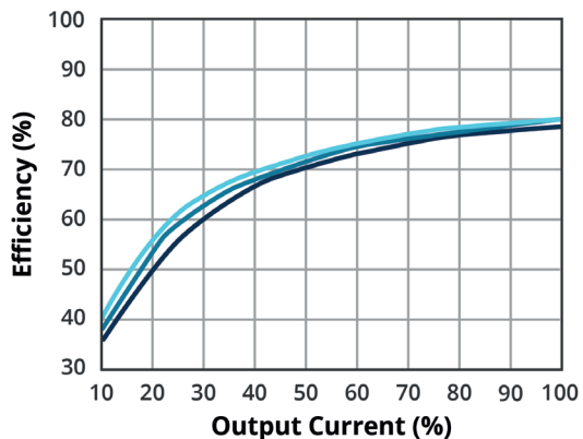
EFFICIENCY VS OUTPUT LOAD PCN1-S5-D12-S
