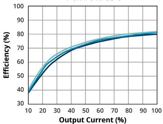
EFFICIENCY VS OUTPUT LOAD PCN1-S12-S5-S
