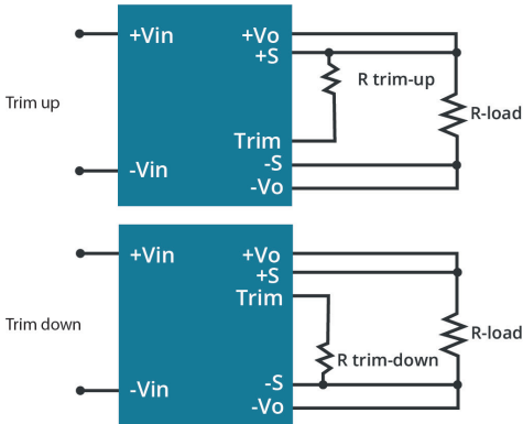
Figure 1 Application Circuit for Trim pin
