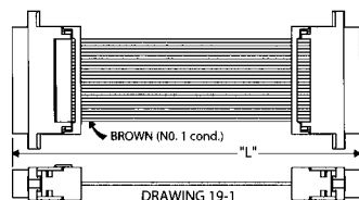
DRAWING 19-1
