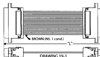
DRAWING 19-3
