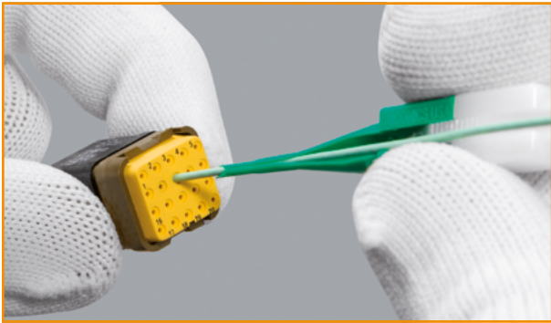
Insert the contact in the module cavity. Push the contact fully home. Then remove the tool and lightly pull back on the wire to make sure that the contact is fully seated.
