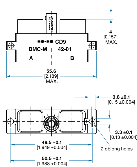
DMC-M 42-01: 2 Modules
