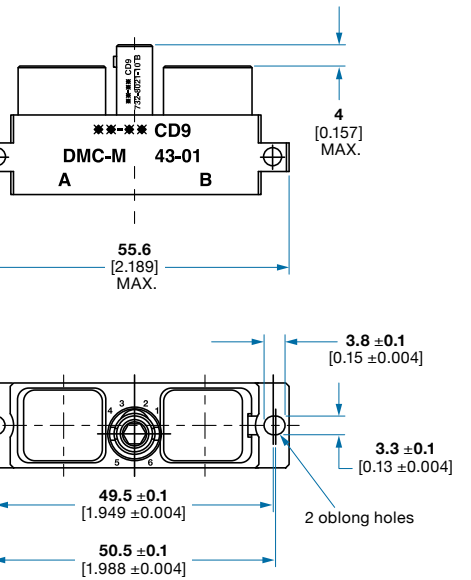
DMC-M 43-01: 2 Modules
