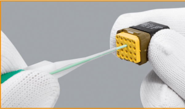
For extraction, insert the wire in the slot of the white end of the tool. Slide the tool into the cavity and push it in until butts against the contact shoulder.
