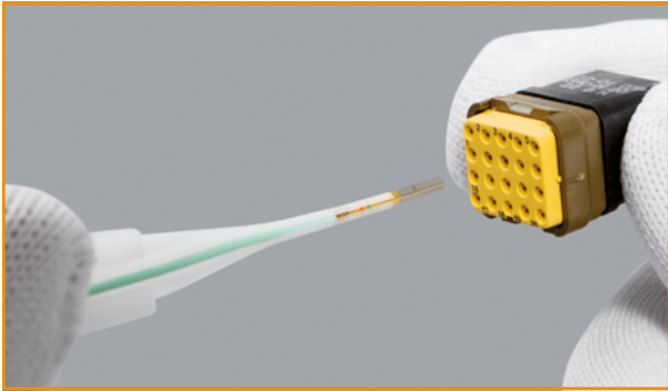
Press the wire between the fingers and the tool. Then pull the overall wire and tool back.
