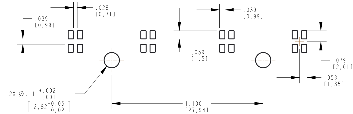
RECOMMENDED SOLDER PAD LAYOUT
