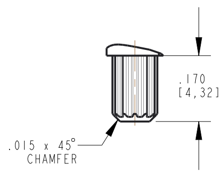
DETAIL A SCALE 4.000
