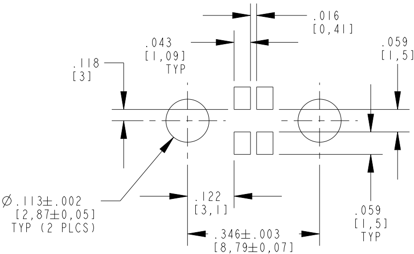
SOLDER PAD AND HOLE LAYOUT FOR BI-COLOR SMT LED (DIALIGHT P/N'S 597-77XI-2XXF)
