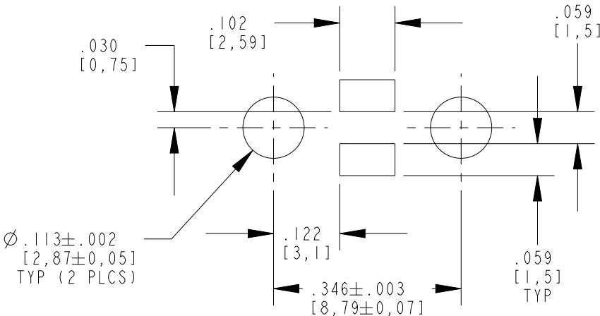
SOLDER PAD AND HOLE LAYOUT FOR SINGLE COLOR SMT LED (DIALIGHT P/N'S 597-3XXI-2XXF)
