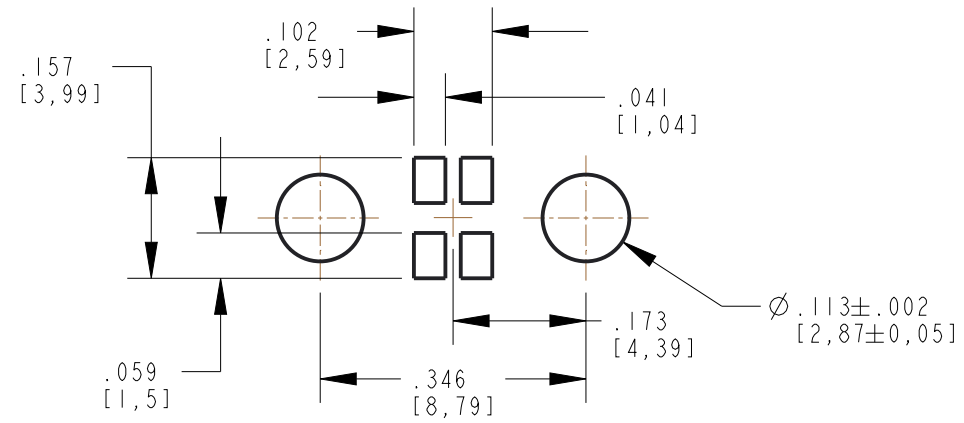
RECOMMENDED SOLDER PAD LAYOUT (MULTI COLOR 597-77X1-207F)
