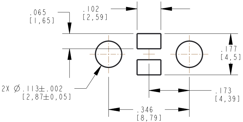
RECOMMENDED SOLDER PAD LAYOUT (SINGLE COLOR 597-3XX1-207NF)
