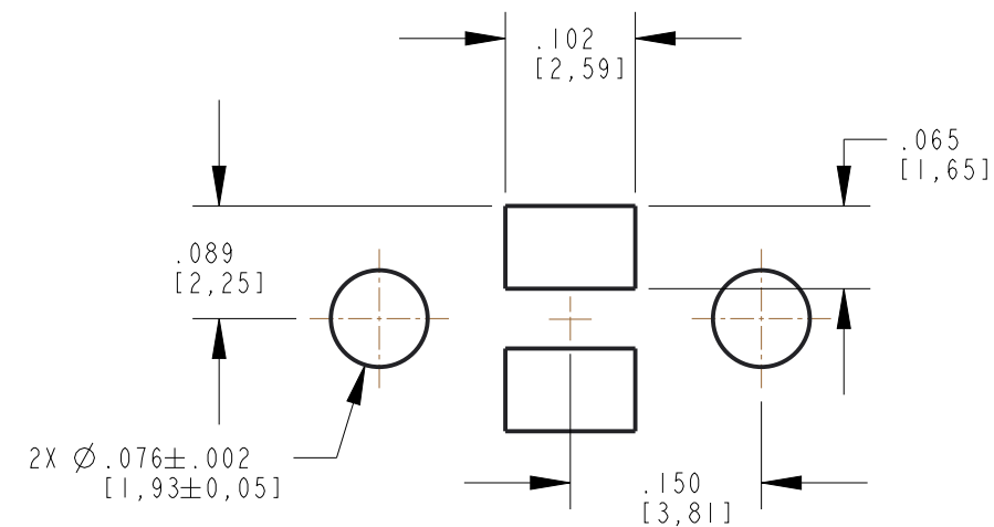
RECOMMENDED SOLDER PAD LAYOUT (SINGLE COLOR 597-3XX1-207NF)
