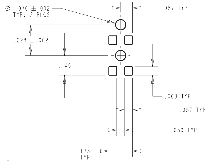
SOLDER PAD/HOLES LAYOUT SINGLE COLOR LED 597-3X11-5XXF
