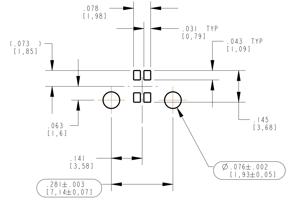
SOLDER PAD/HOLE LAYOUT FOR BI-COLOR
