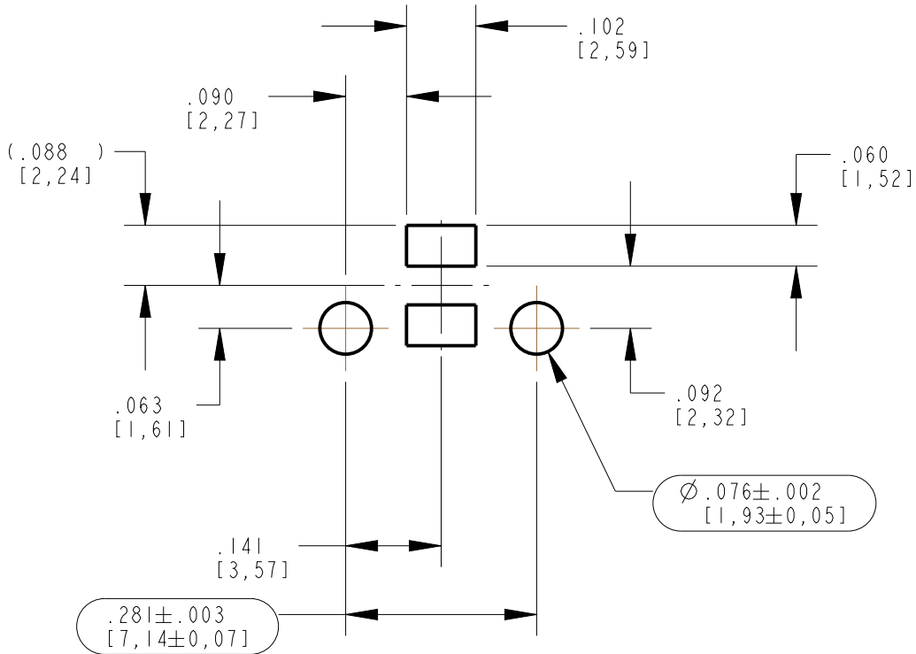
SOLDER PAD/HOLE LAYOUT FOR SINGLE COLOR SCALE 4.000
