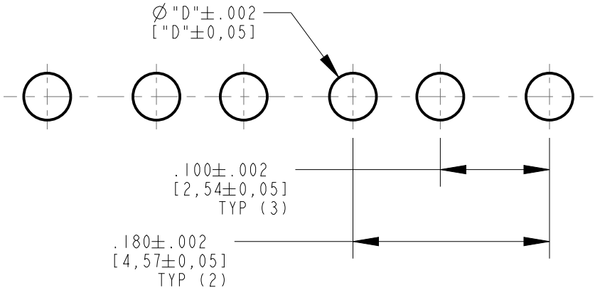
RECOMMENDED HOLE PATTERN
