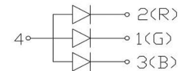
LED SCHEMATIC
