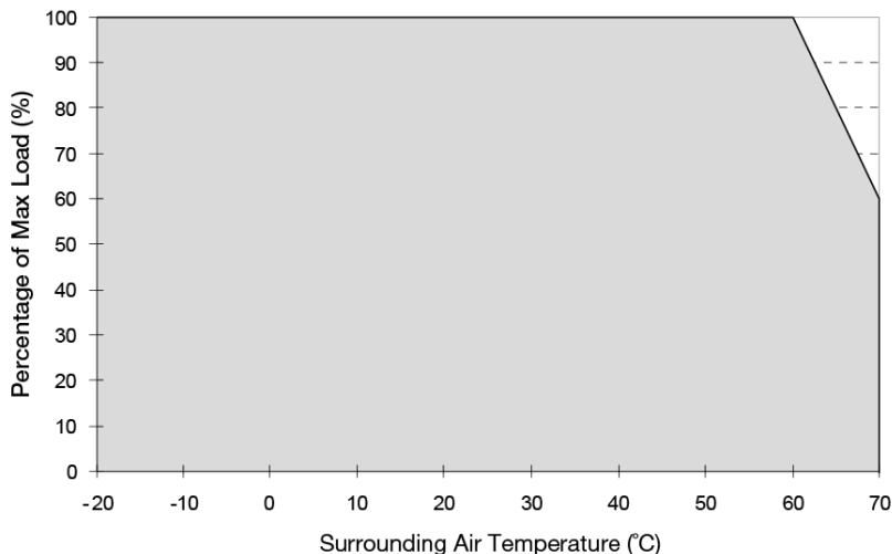
Fig. 1 De-rating for All Mounting Orientation (All Models) > 60°C de-rate power by 4% / °C
