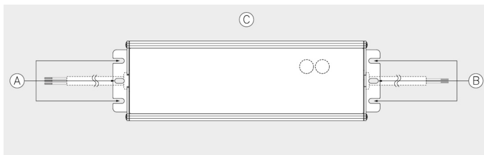
Fig. 3 Mounting Hole Locations
