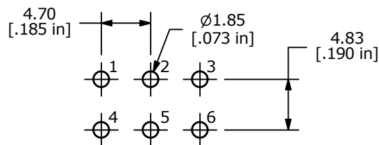
PC MOUNTING
