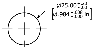
RECOMMENDED PANEL CUTOUT MAX. PANEL THICKNESS 10.0 [0.39 in]
