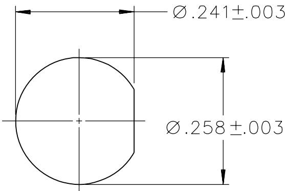
BULKHEAD MOUNTING HOLE 5:1
