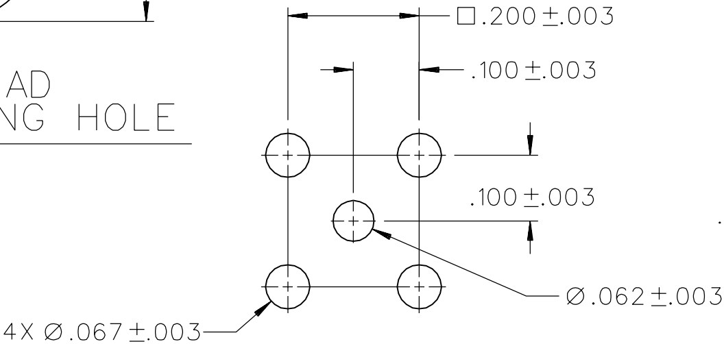
PC MOUNTING HOLE LAYOUT 5:1
