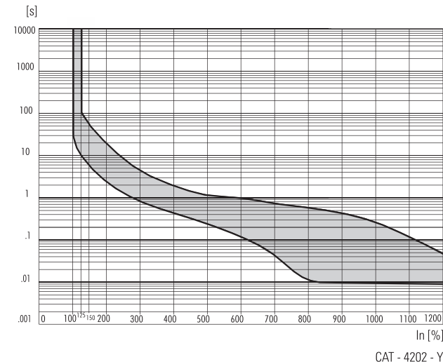
Curve 20 50/60 Hz
