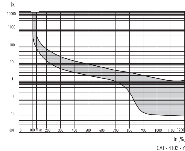
Curve 10 50/60 Hz
