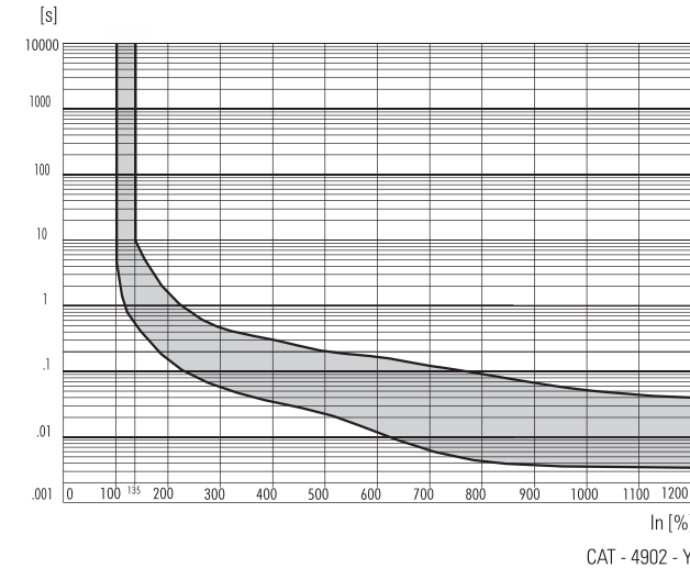
Curve 30 50/60 Hz/DC
