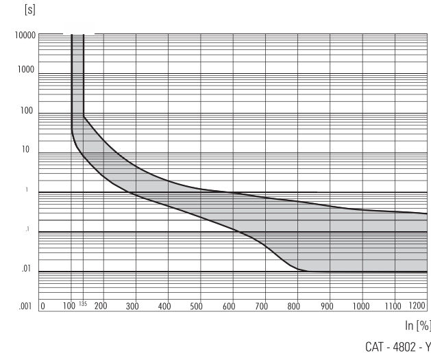
Curve 20 50/60 Hz/DC
