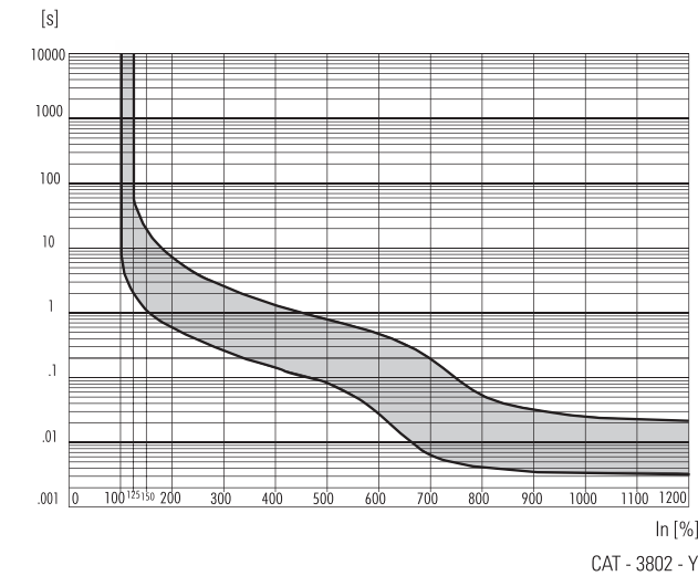
Curve 3 400 Hz
