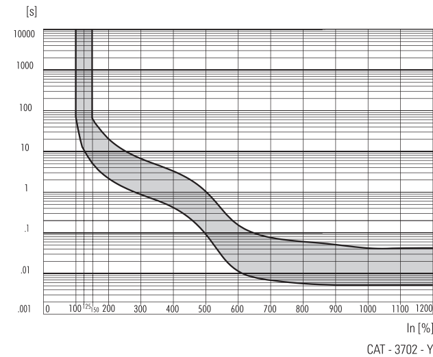
Curve 2 400 Hz
