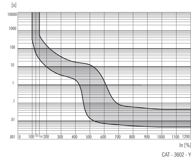
Curve 1 400 Hz
