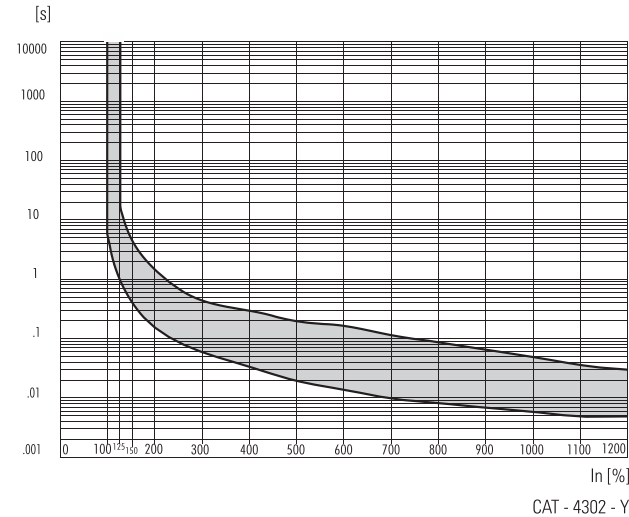
Curve 30 50/60 Hz
