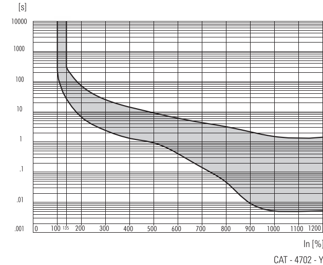
Curve 10 50/60 Hz/DC
