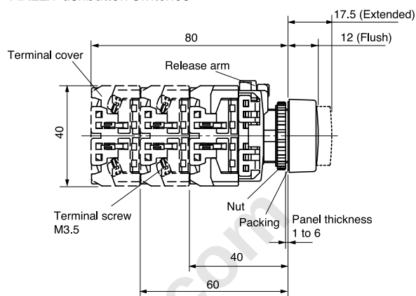
AR22/Pushbutton switches
