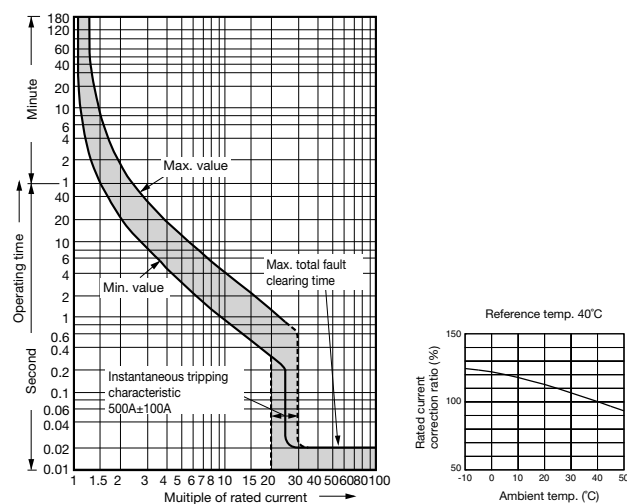
● BW125, EW125 (Rated current: 20A)
