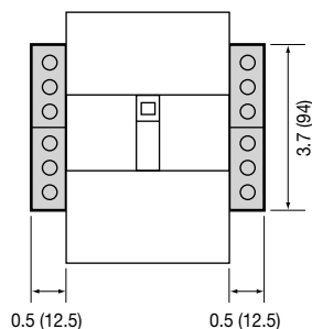
Dimensions of Undervoltage/Shunt trip device 50 and 100AF Only
