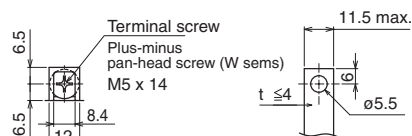
Terminal section detail
