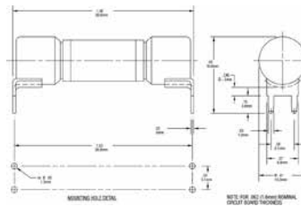
MOUNTING HOLE DETAIL
