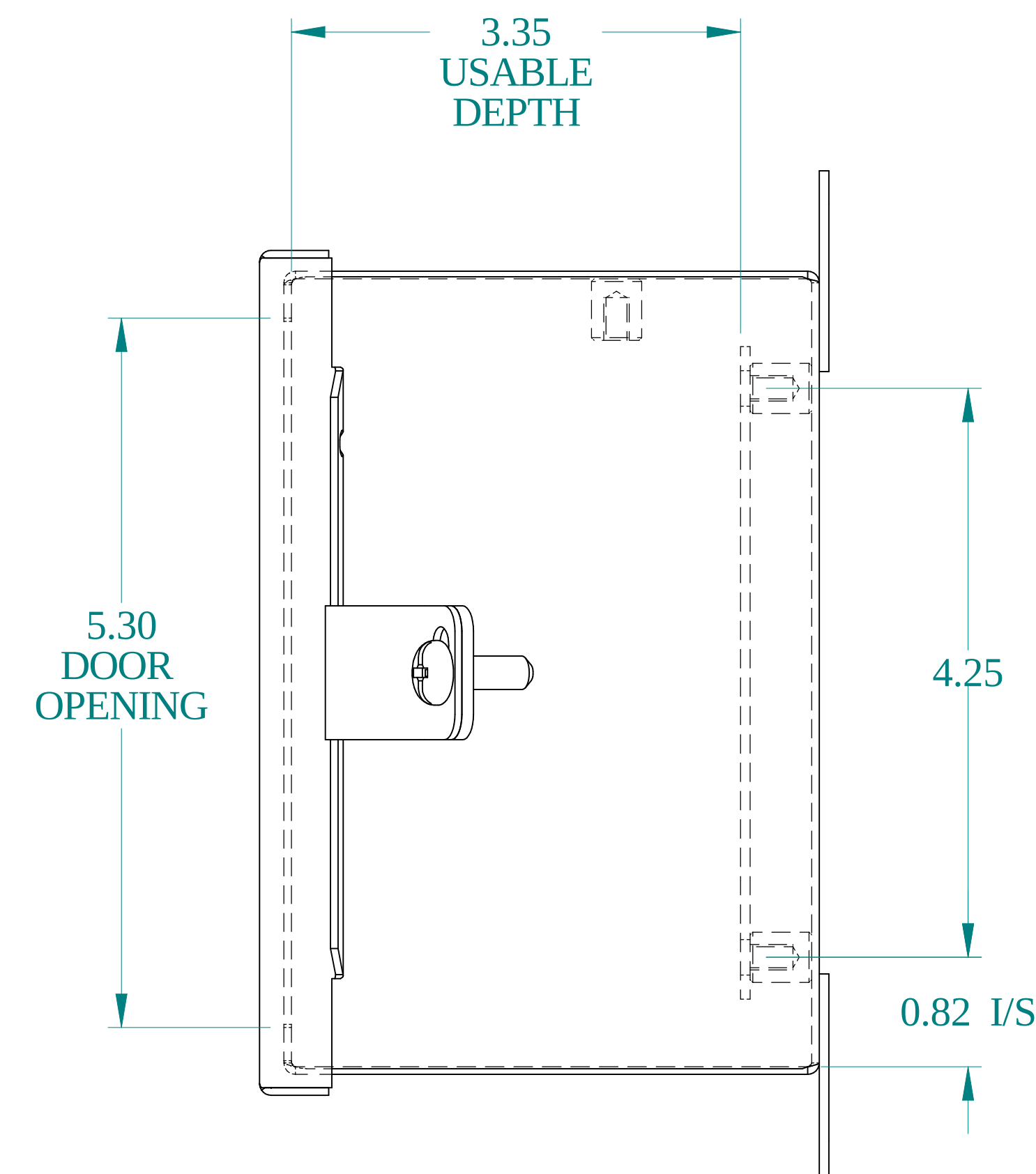
SIDE VIEW
