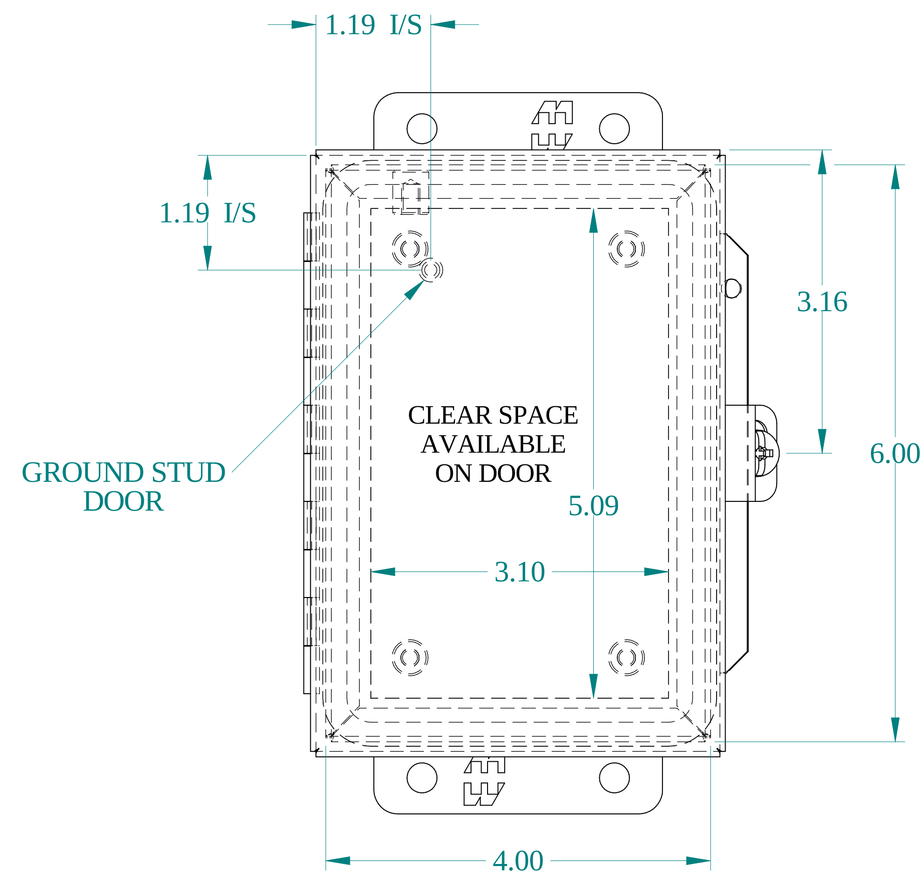
FRONT VIEW
