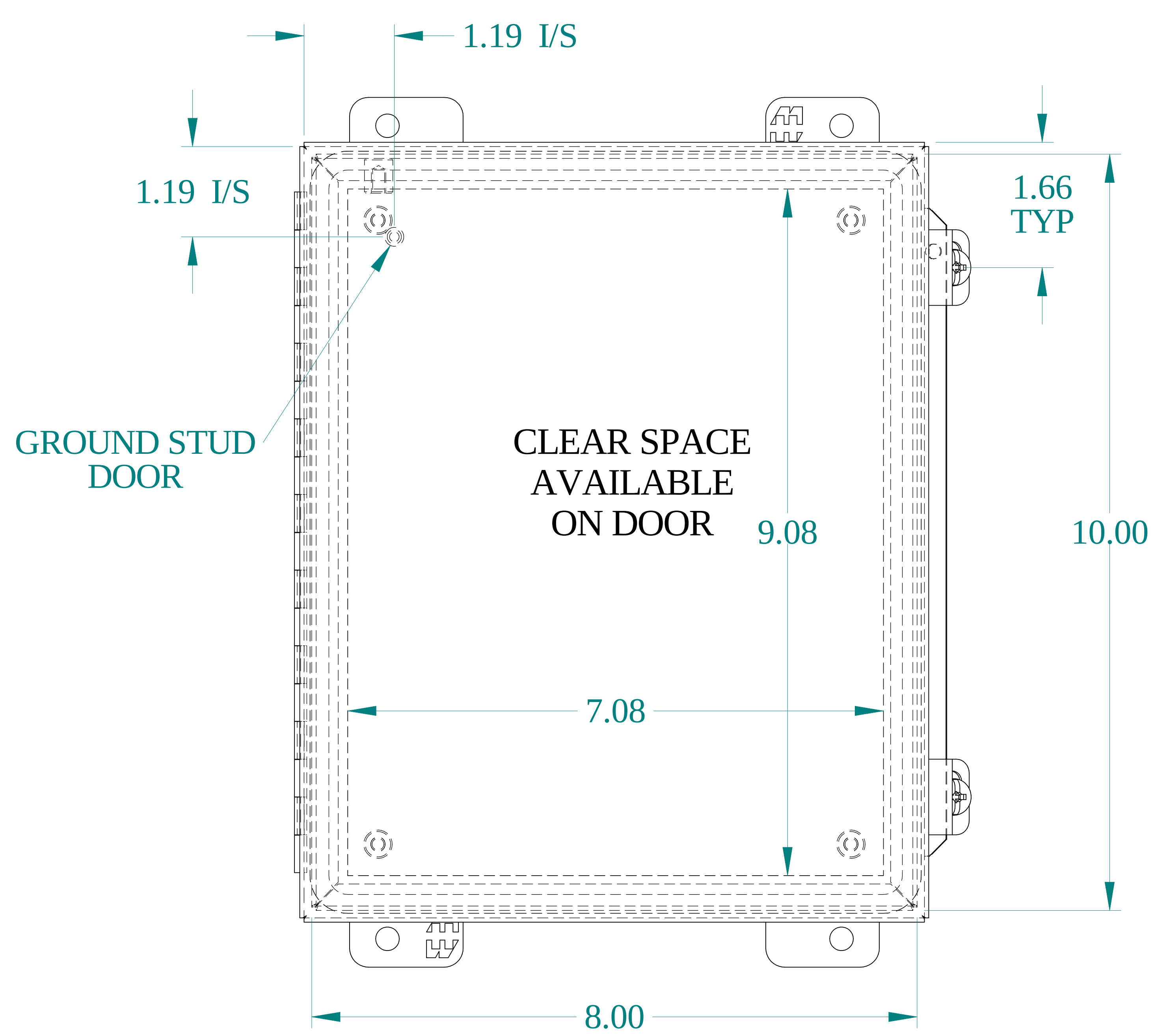
FRONT VIEW
