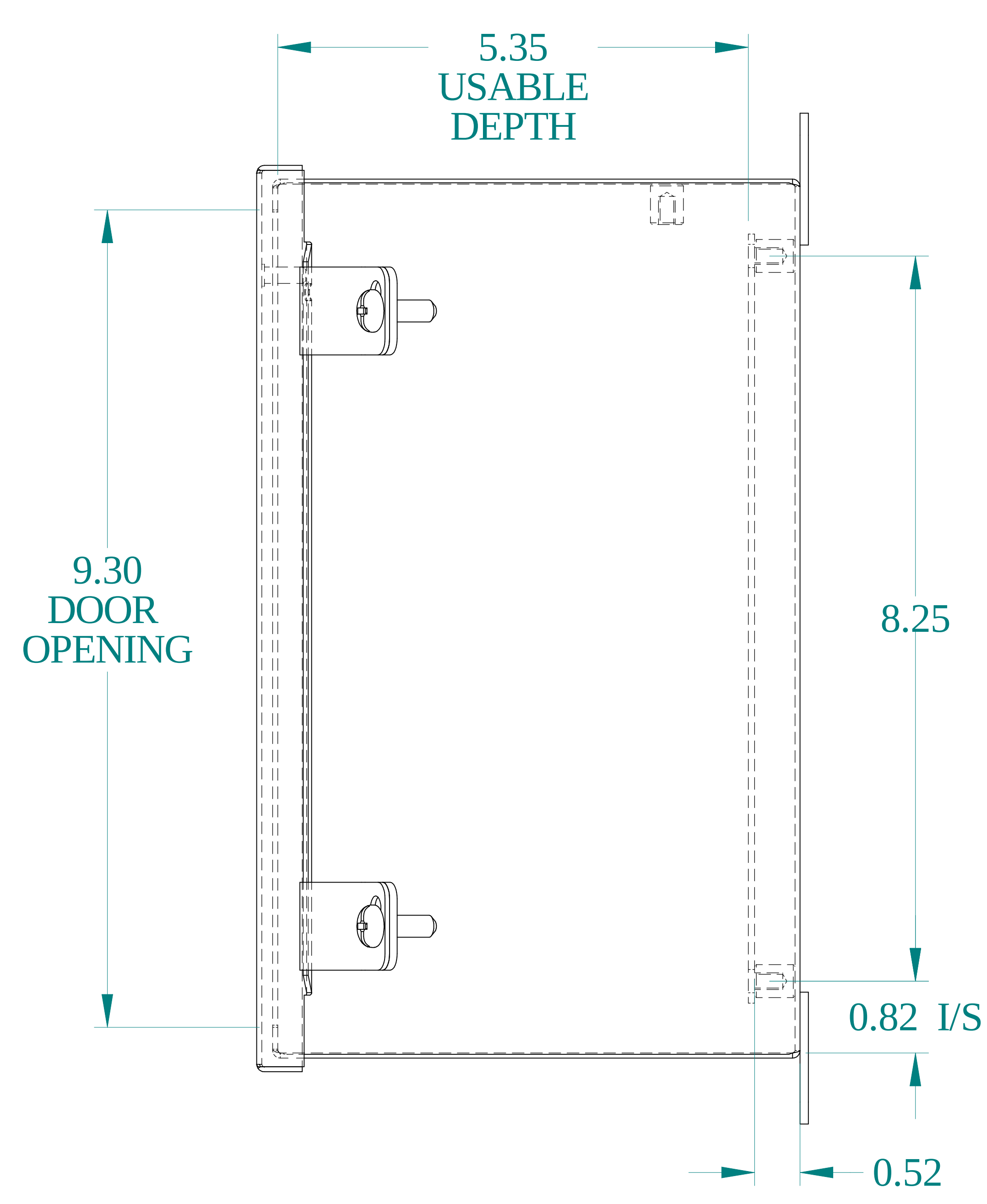
SIDE VIEW
