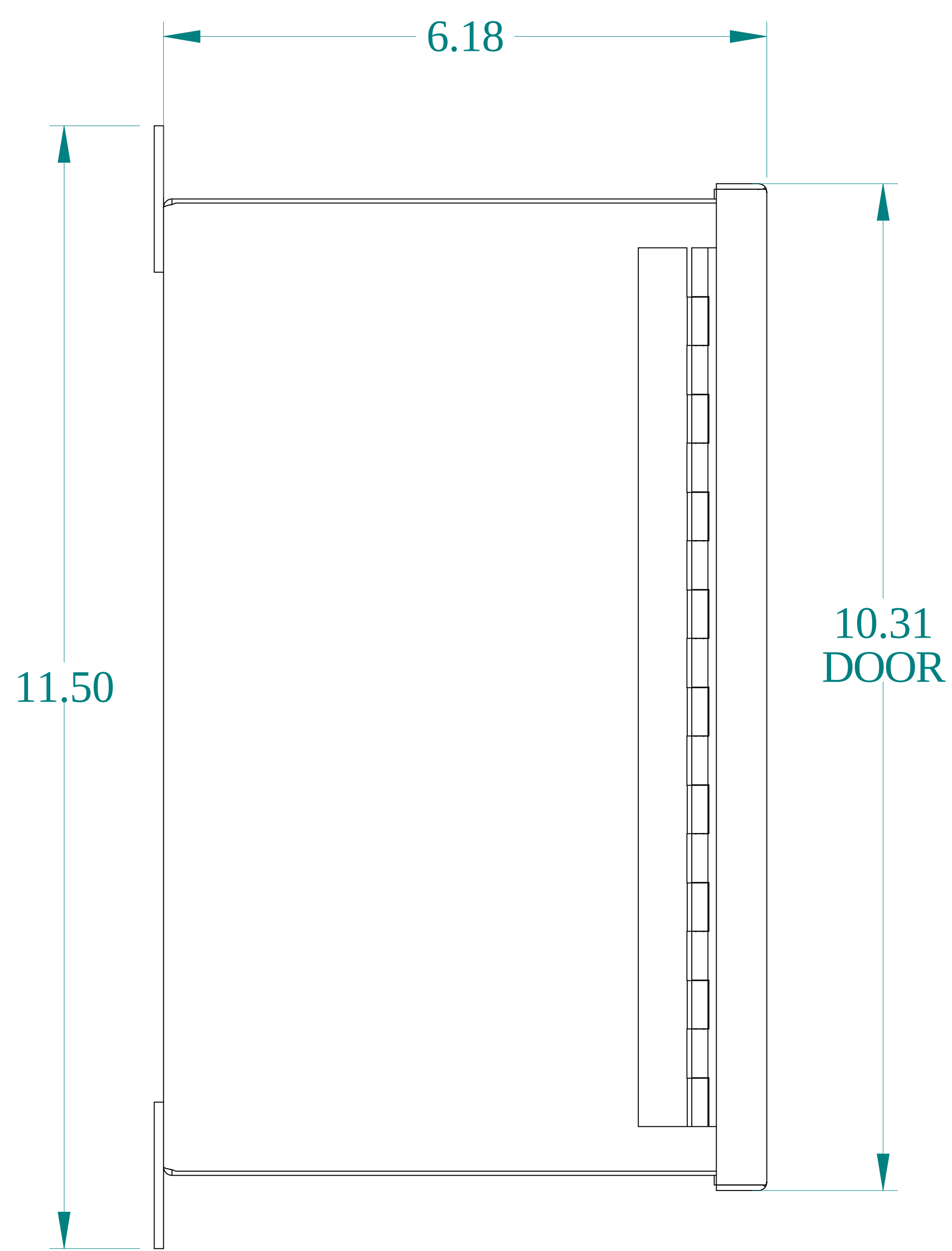
SIDE VIEW
