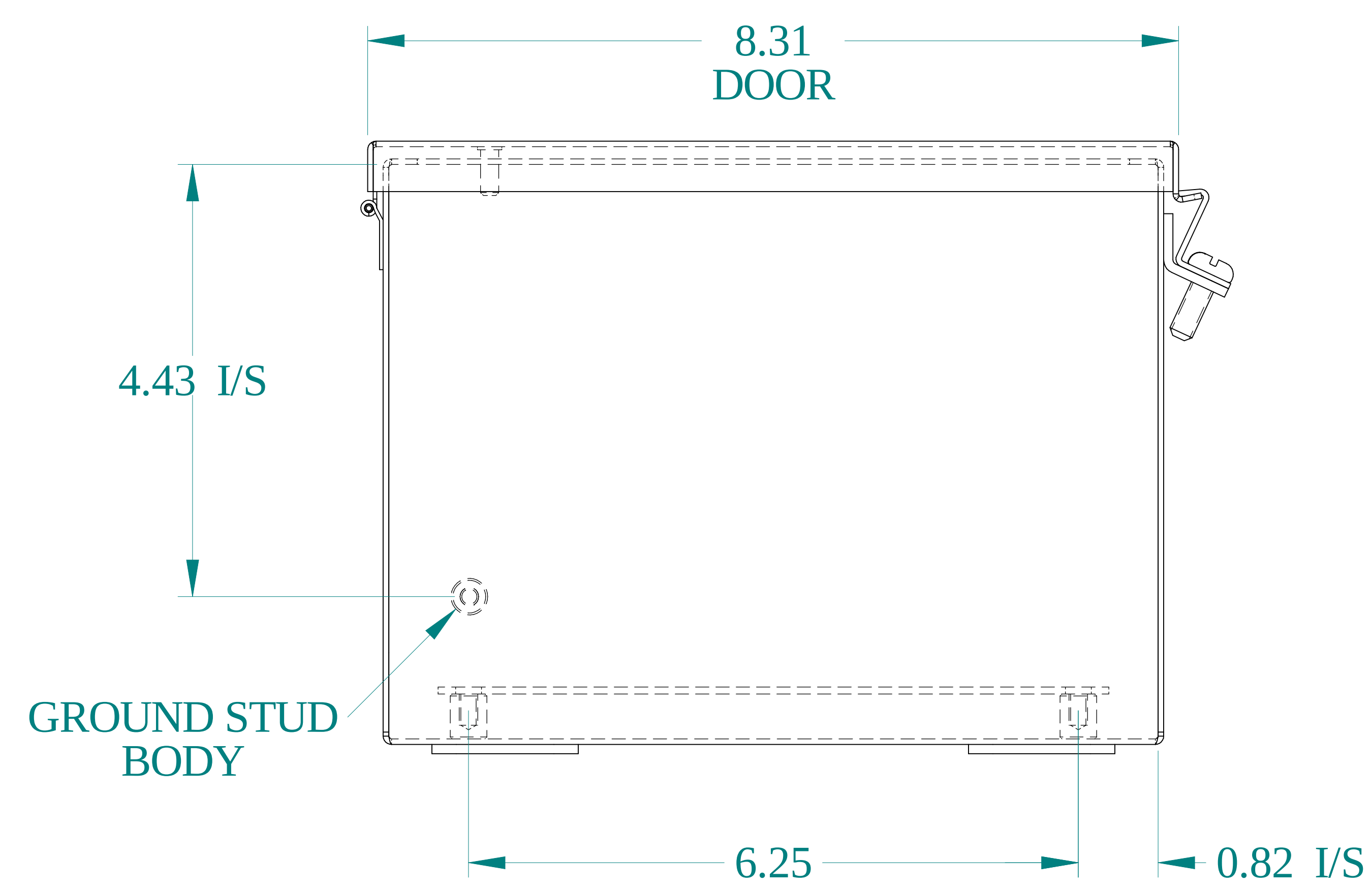
BOTTOM VIEW
