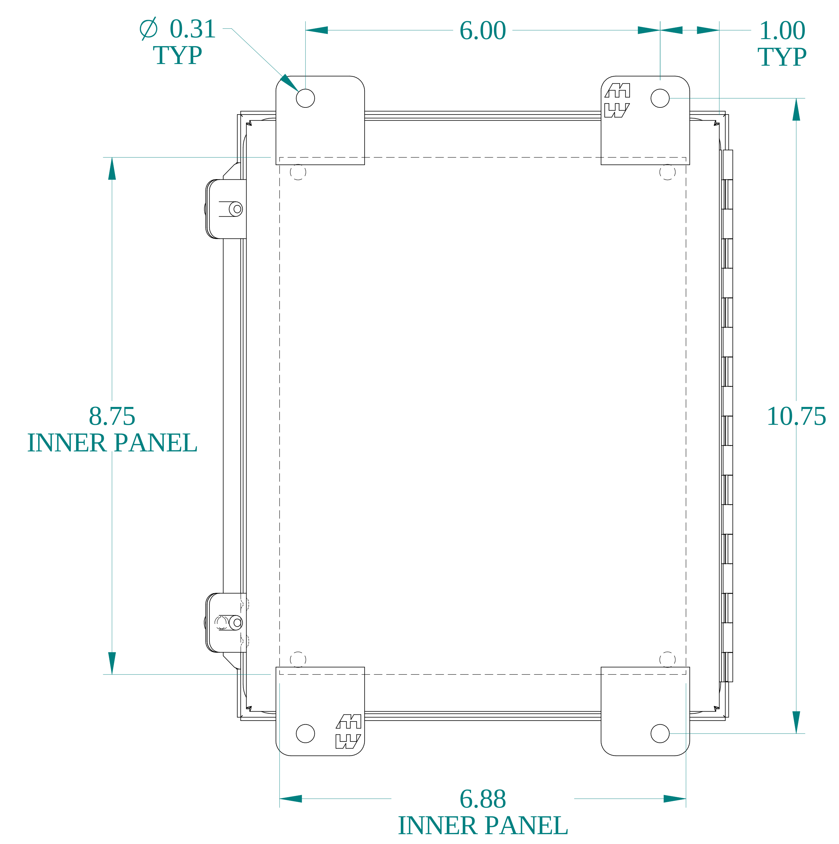
BACK VIEW
