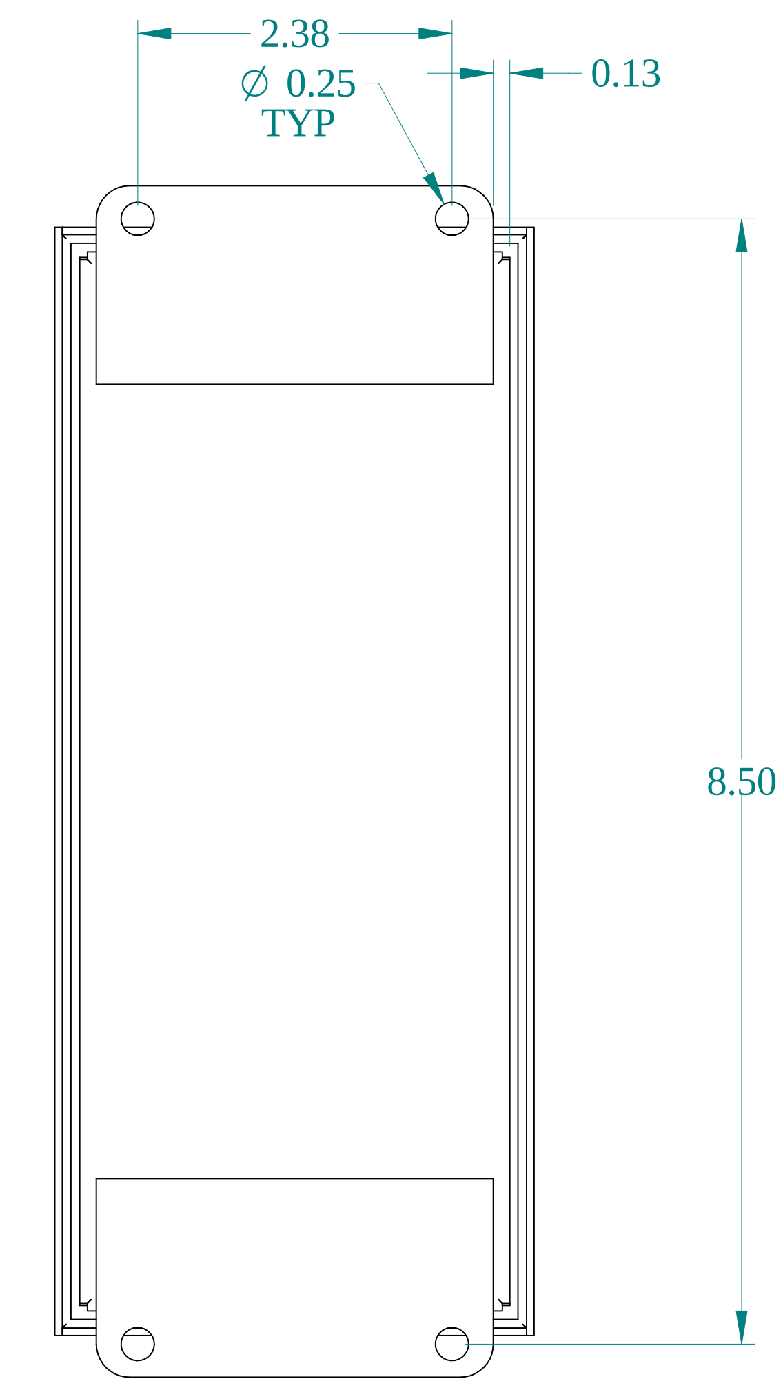
BACK VIEW
