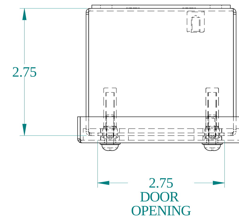
TOP VIEW
