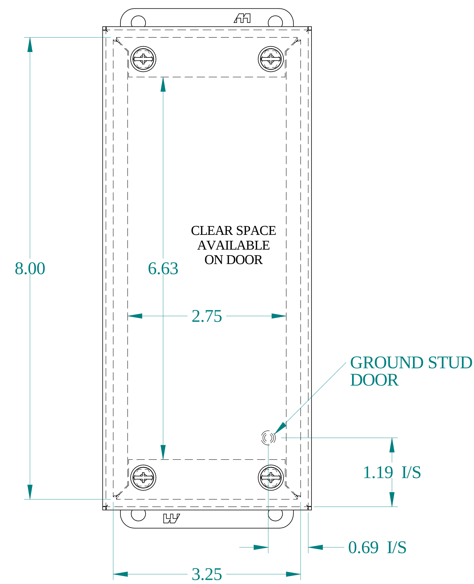
FRONT VIEW
