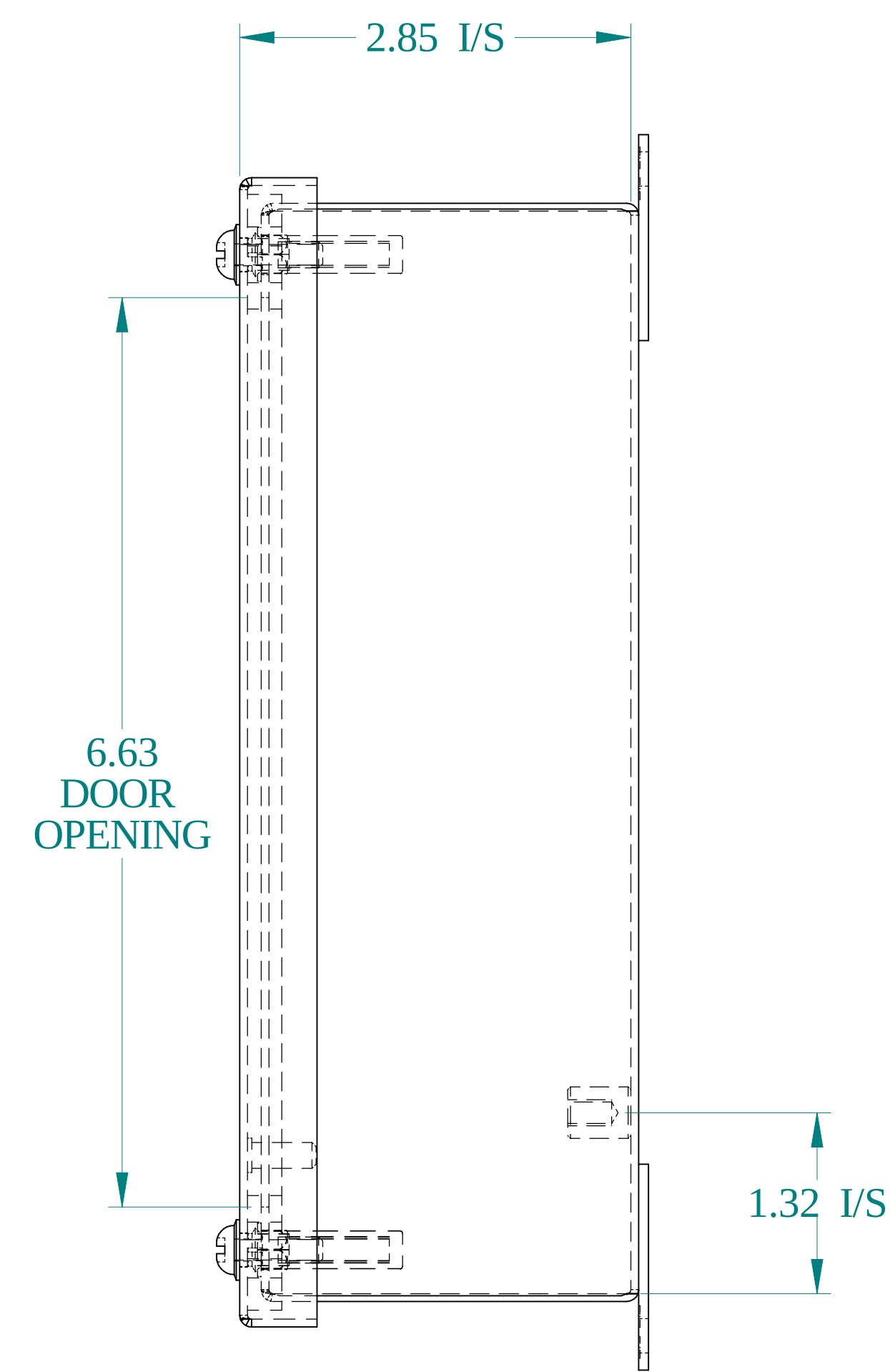
SIDE VIEW
