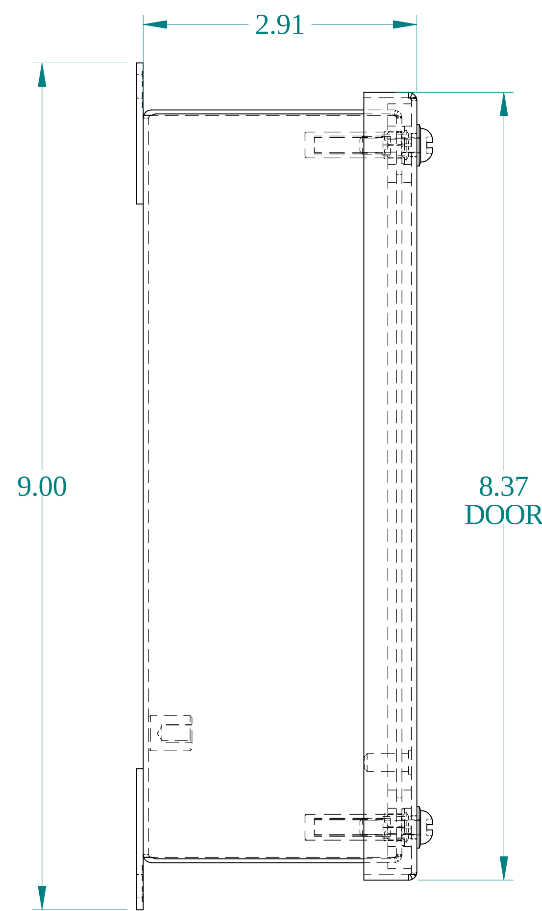
SIDE VIEW
