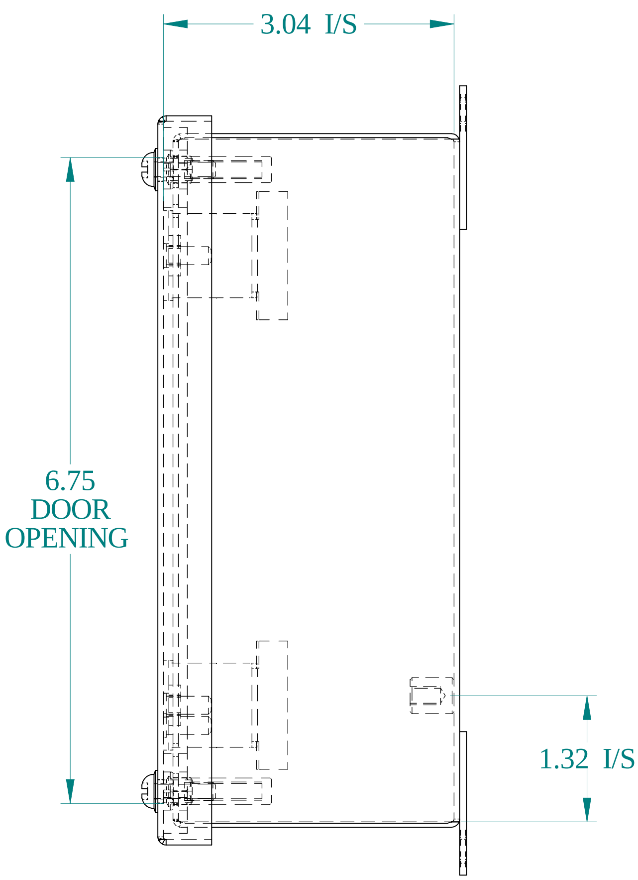
SIDE VIEW
