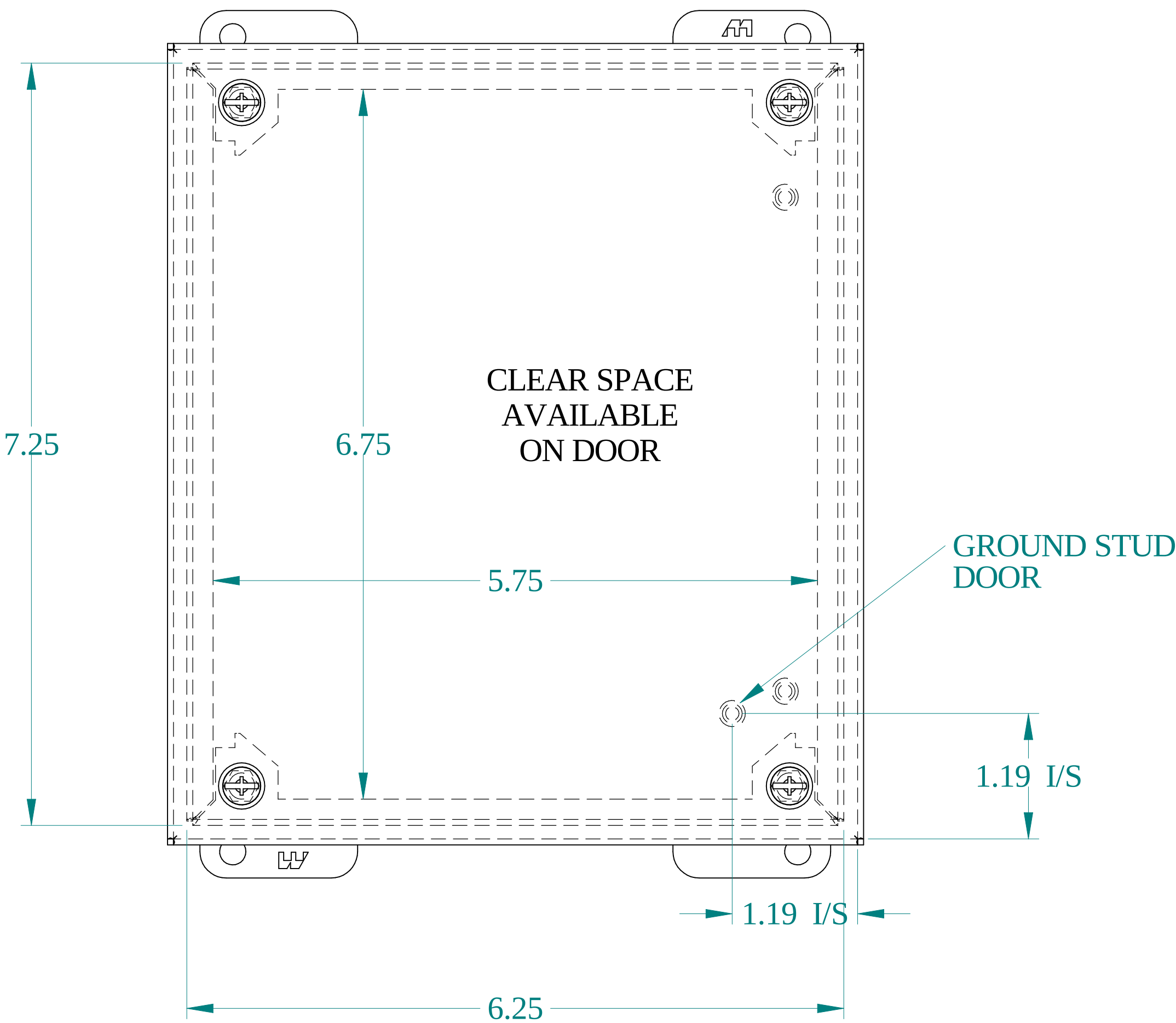
FRONT VIEW
