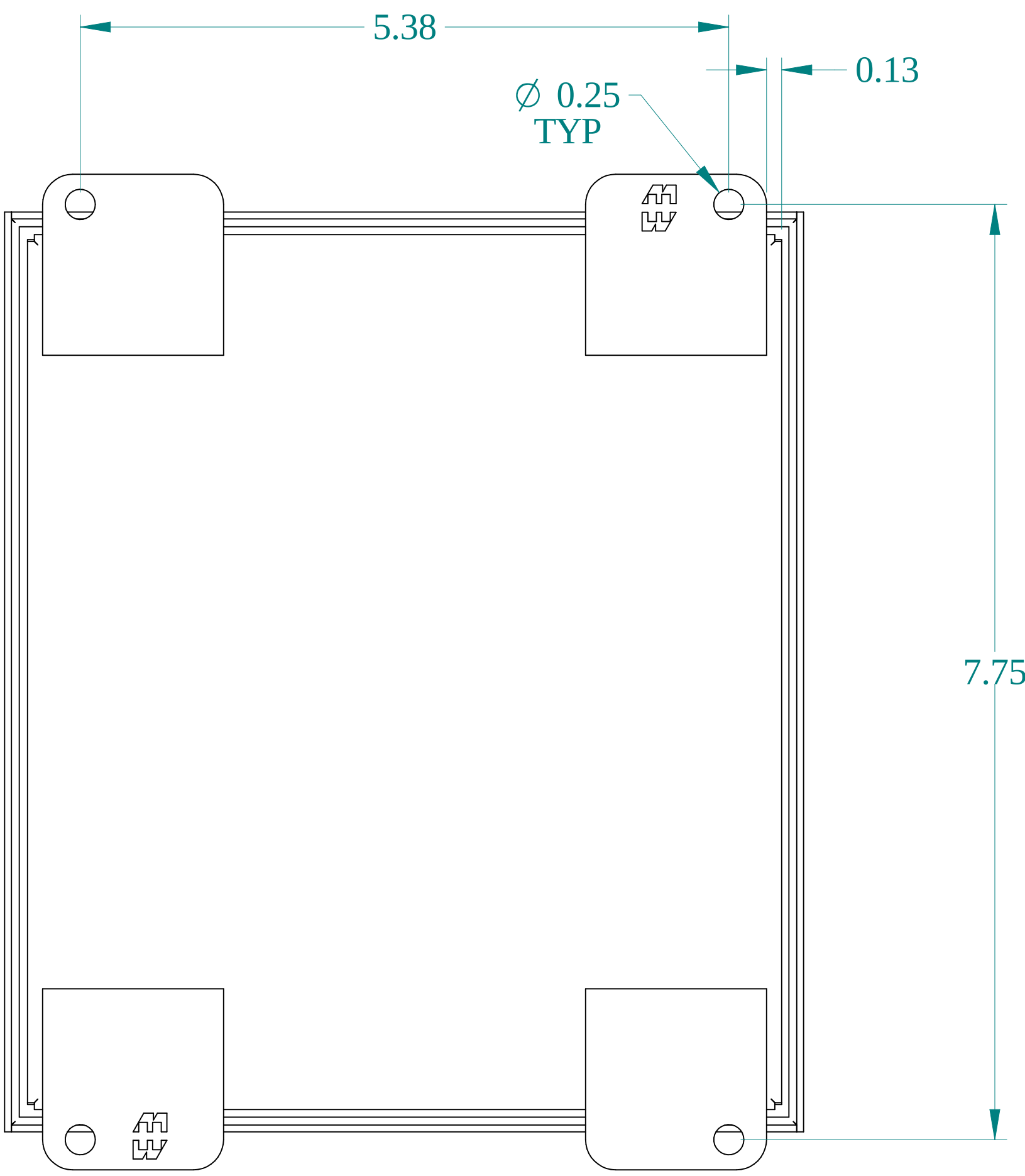
BACK VIEW
