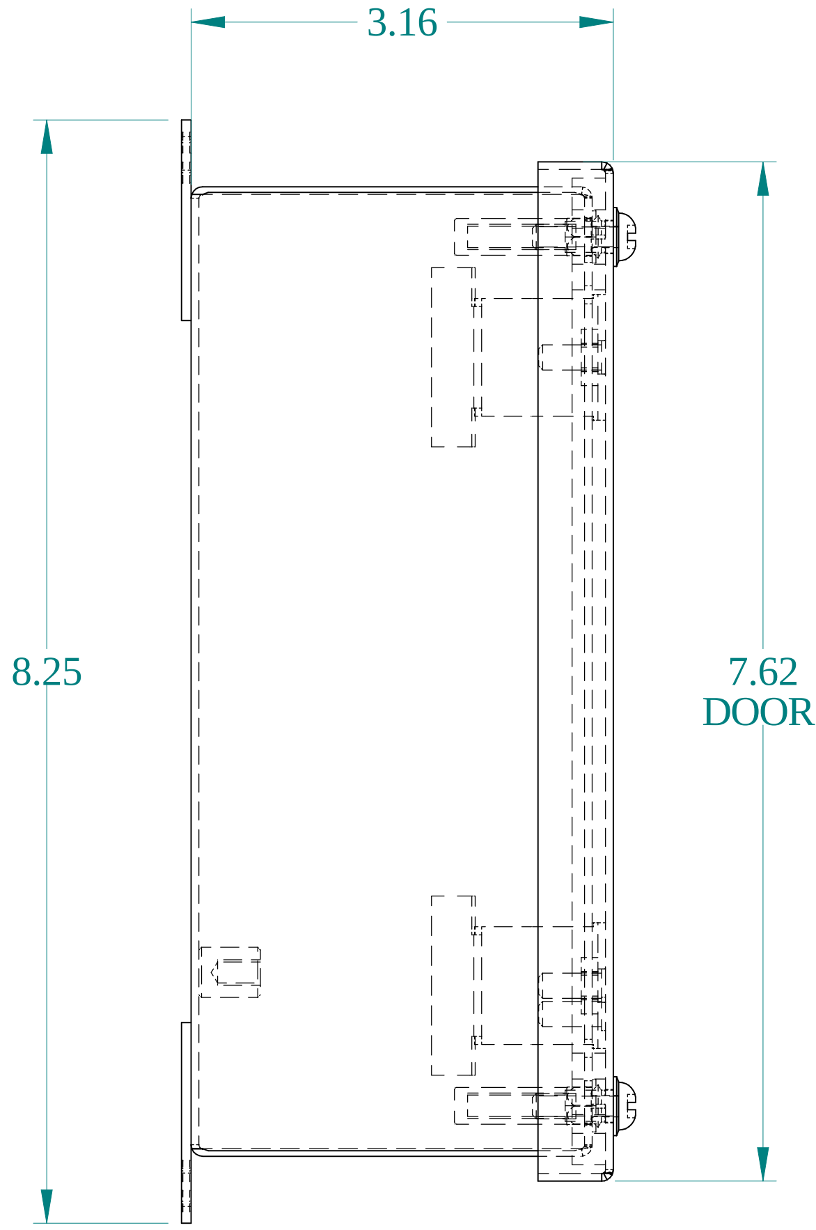
SIDE VIEW
