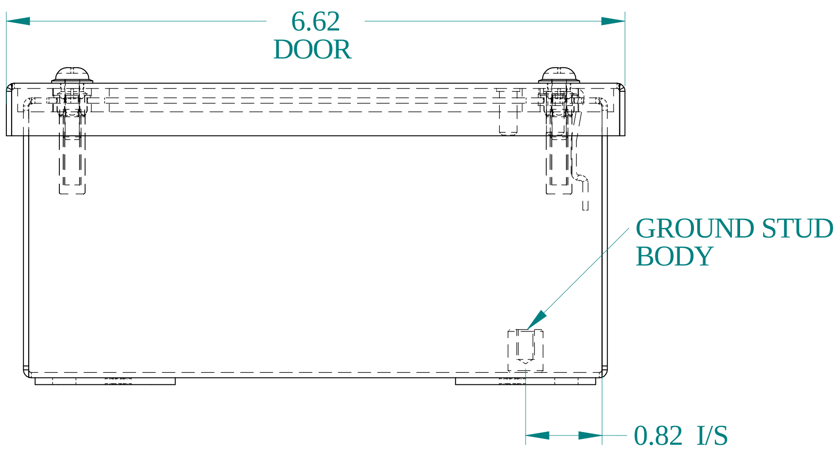
BOTTOM VIEW
