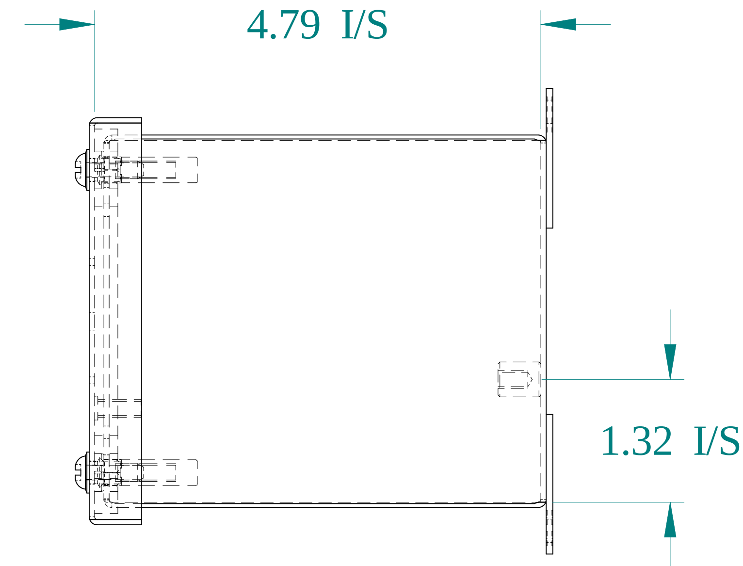
SIDE VIEW
