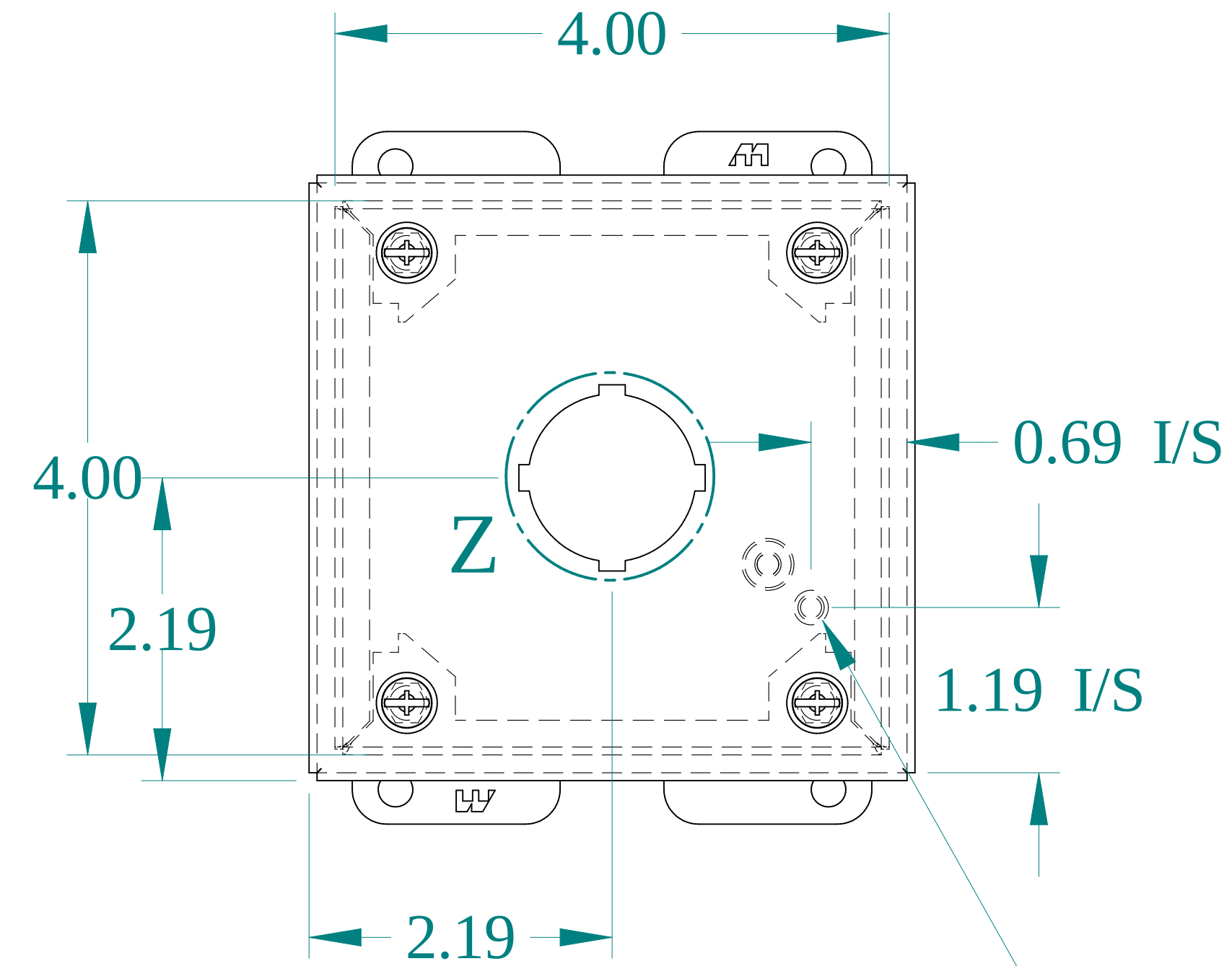
FRONT VIEW
