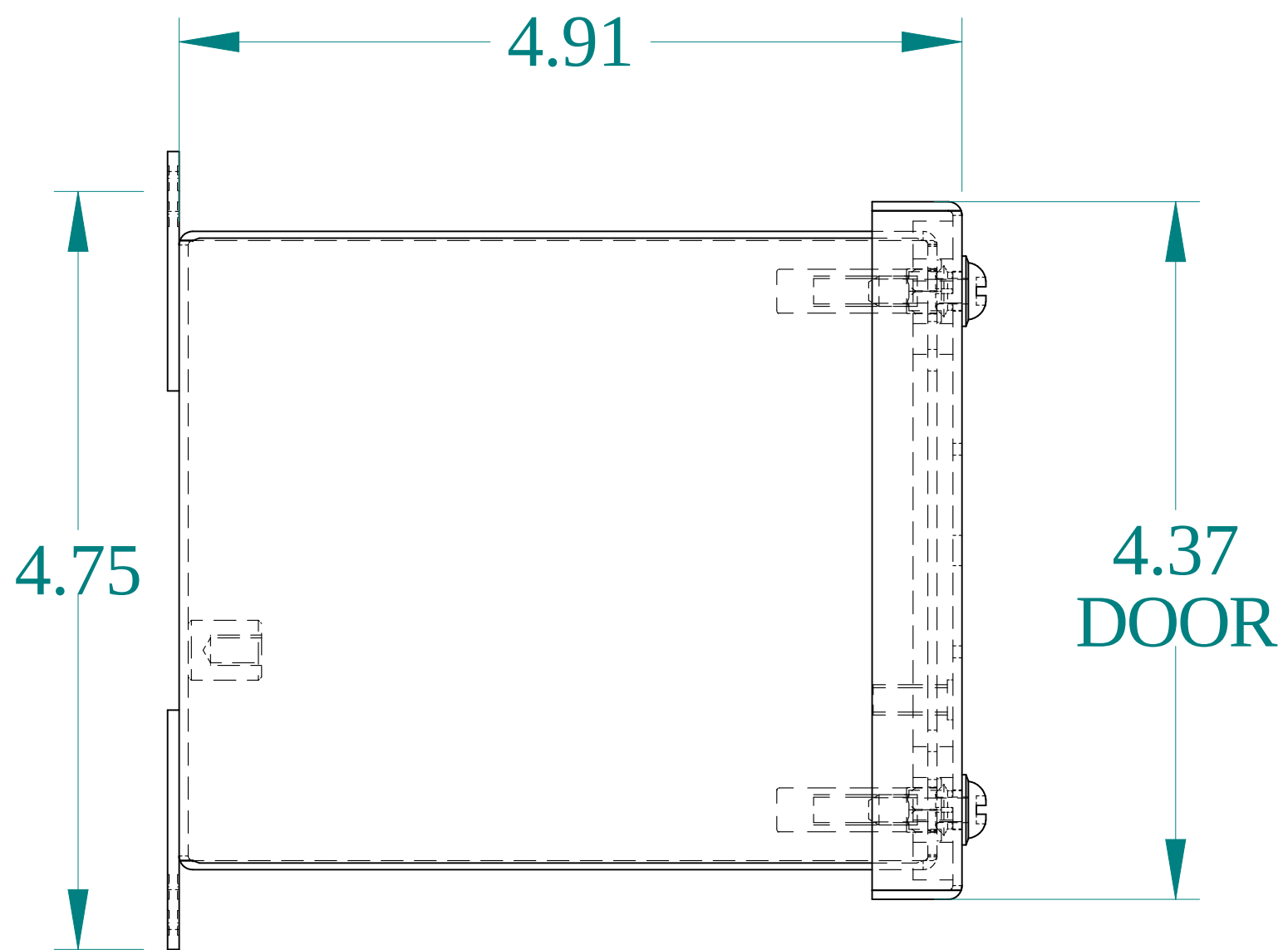
SIDE VIEW
