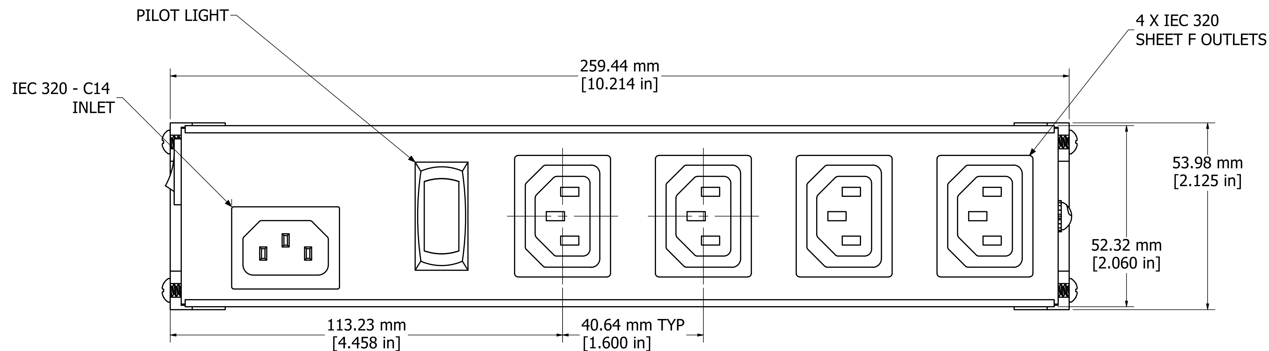
ASSEMBLY - VIEW FROM TOP
