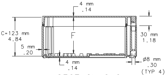
SECTION C-C
