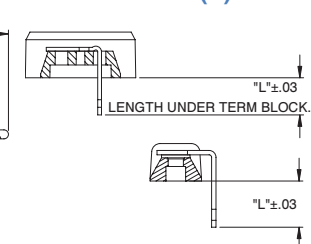
DETAIL (R)
