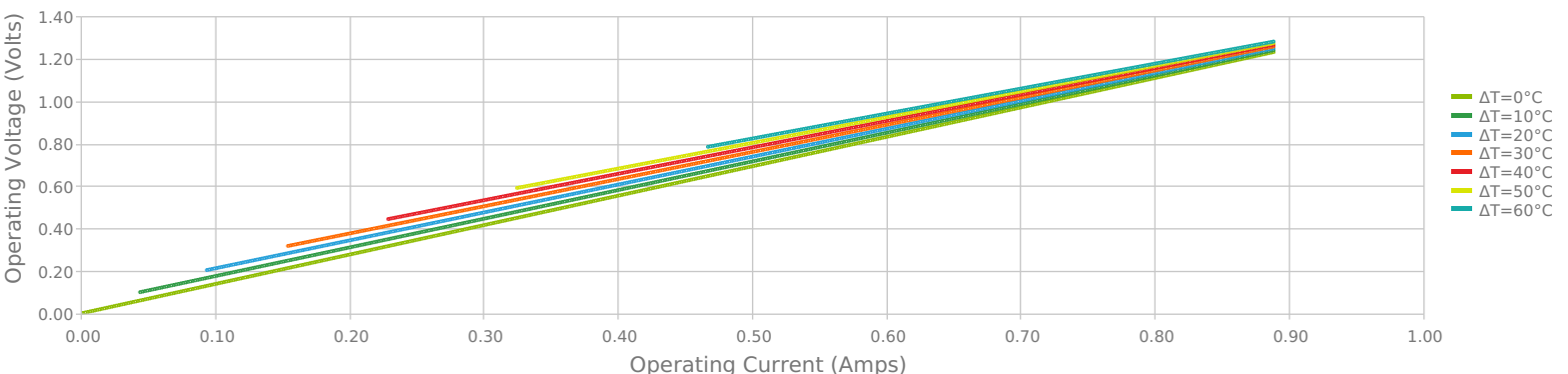
Current vs Voltage (I vs V) T_{hot} = 27\text{ }^{\circ}\text{C}
