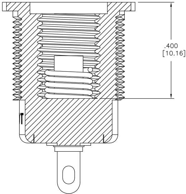
SECTION A-A (WITHOUT HARDWARE) SCALE 4:1
