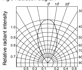
Fig.6 Radiation diagram
