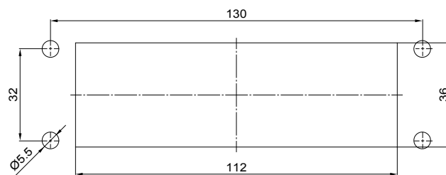
Hole Dimensions
