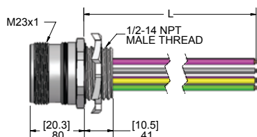
1/2"-14 NPT Thread
