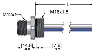
Male Receptacle
