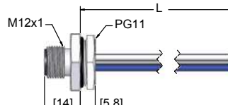
Male Receptacle
