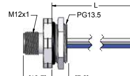
Male Receptacle
