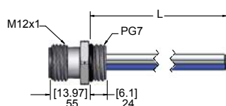
Male Receptacle
